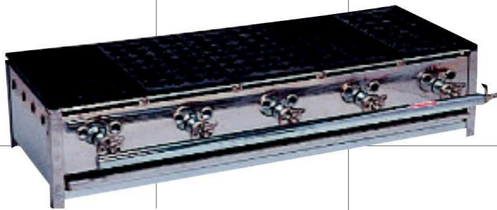
■ Takoyaki machine 84 rolls W560×D350×H230mm ■ Takoyaki machine 140 rolls W970×D340×H230mm
